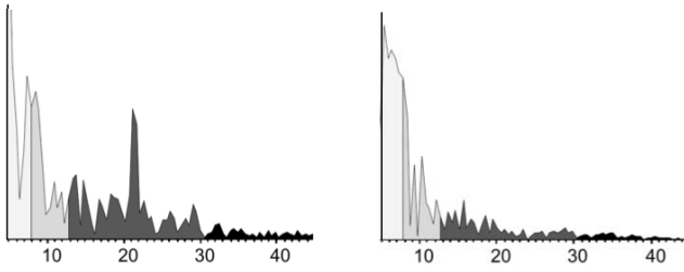
Figure 2: Fast fourier transform (FFT) of the ERP from the P7 and P8 electrode locations for the RSVP (left) and Onset (right) condition. The RSVP condition shows a peak in the FFT plot at the frequency of target presentation (approx. 21Hz), which is not present for Onset presentation.
