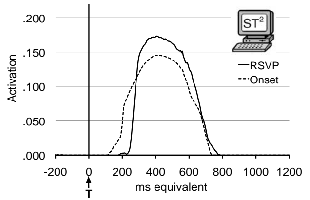
Figure 6: After Step 3: Virtual P3 for the RSVP and Onset condition. The RSVP vERP is baseline corrected to -200 to 0ms with respect to target onset to account for distractor related activity, which is absent in the Onset condition. ERPs are time-locked to target presentation time ‘T’.
