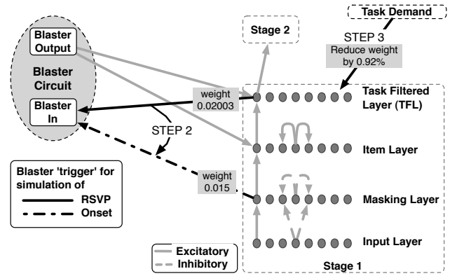
Figure 4: Steps 2 and 3 of simulating Onset presentation. In Step 2, the connection that triggers the blaster is moved from the TFL to the masking layer. In Step 3, the weight of the connection from task demand to target nodes in the TFL is reduced by 0.92%.
