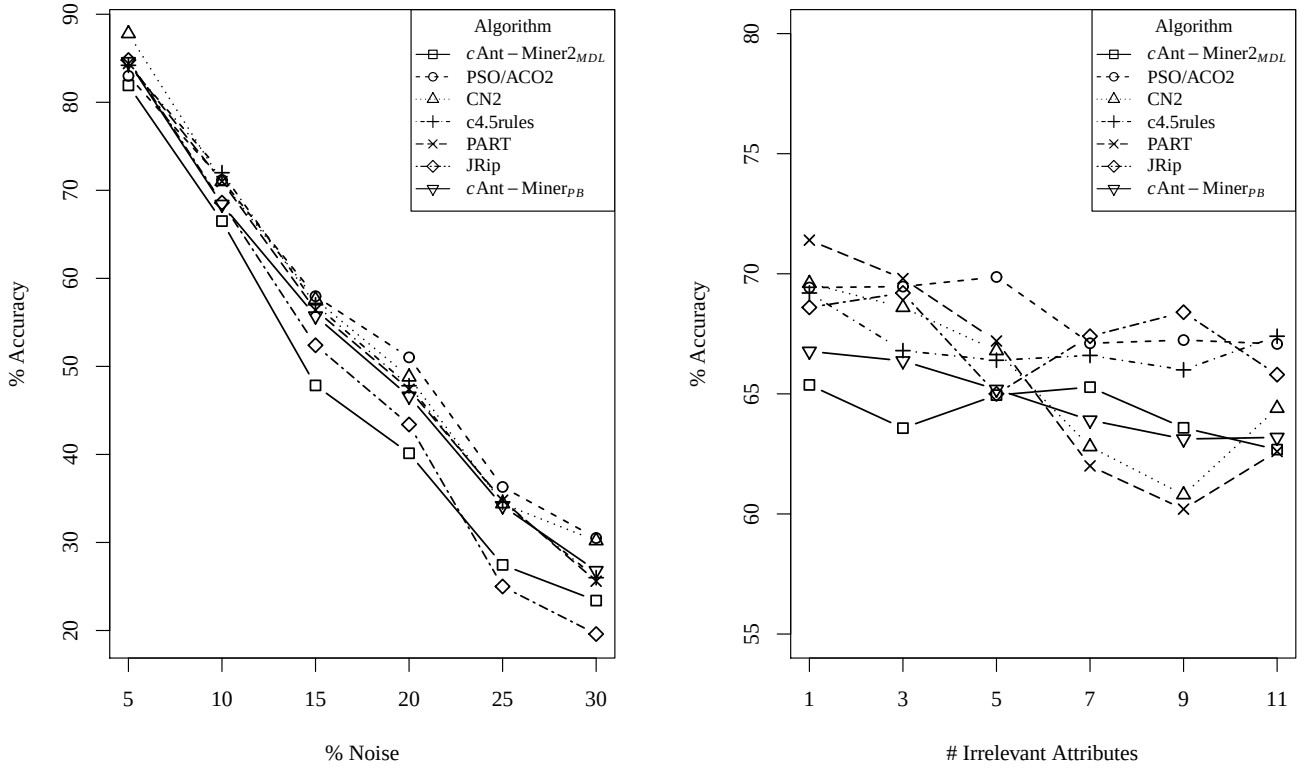
Fig. 4. Performance (measured in terms of predictive accuracy) of the algorithms used in our experiments when presented with irrelevant attributes and noisy data. The graph on the left corresponds to the observations in the data sets with increased noise probability. The graph on the right corresponds to the observations in the data sets with increased number of irrelevant attributes.
