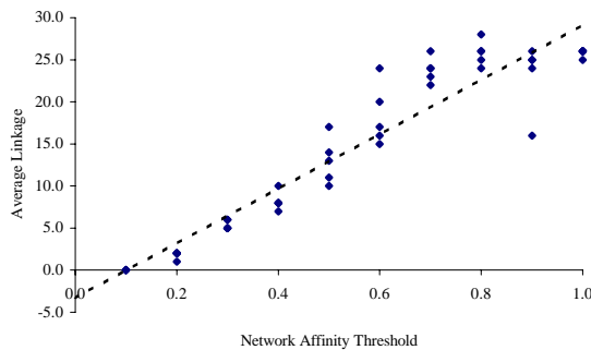
(c) Network after 10 iterations clearly showing a positive correlation between NAT Scalar and network connectivity.
