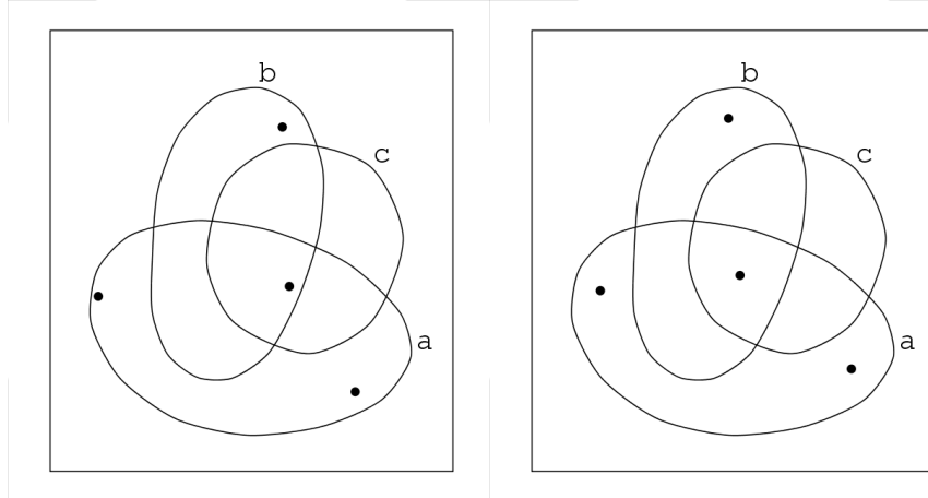
Fig. 8. Initial placement of spider feet (left) and refinement under the force model (right).
