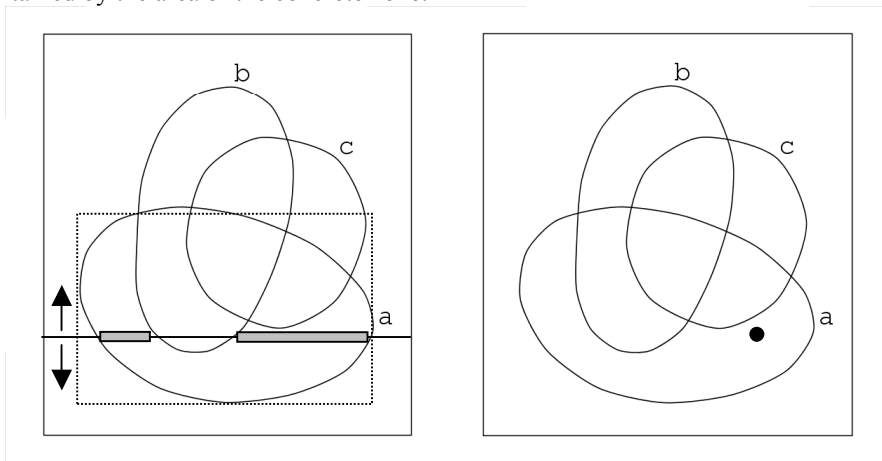
Fig. 7. Candidate locations for a new node in zone a excluding b,c . The horizontal line is placed such that it intersects the bounding box of zone a at a random height. This diagram shows two subintervals where it is valid to place the new node.
