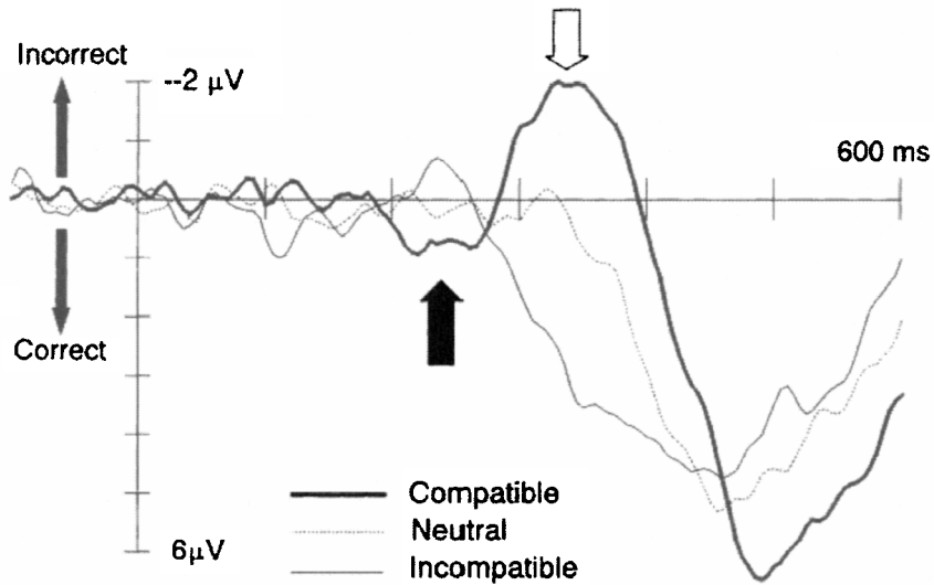
Figure 2. LRP for masked priming task (from Eimer, 1999).
