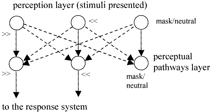
Figure 6. Perceptual system.
