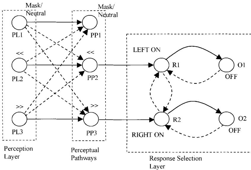
Figure 12. The model.
