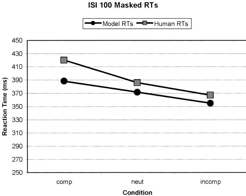
Figure 19. Model and human RT data for basic experiment (human RTs from Eimer & Schlaghecken, 1998, Exp. 1a).
