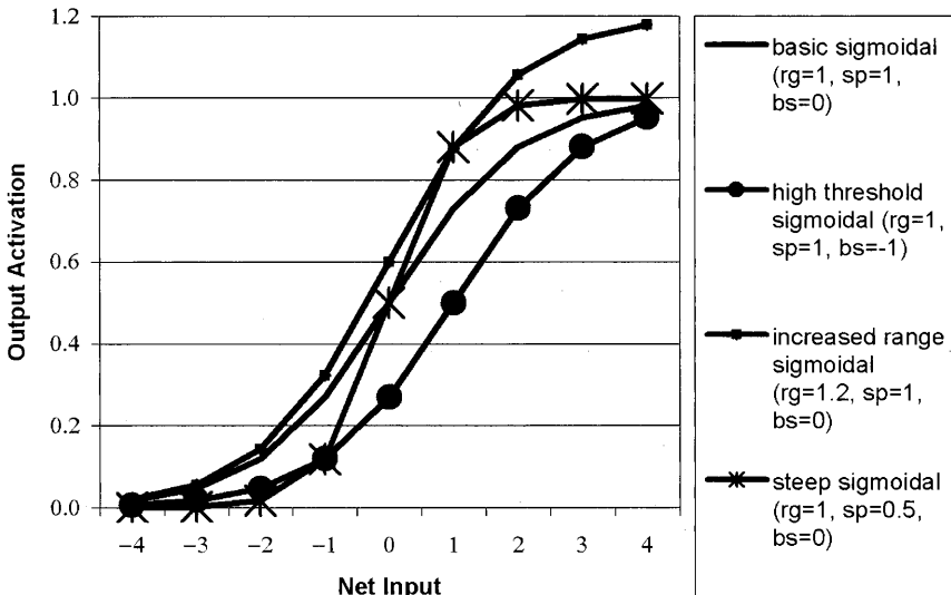
Figure 13. Sigmoidal activation function.
