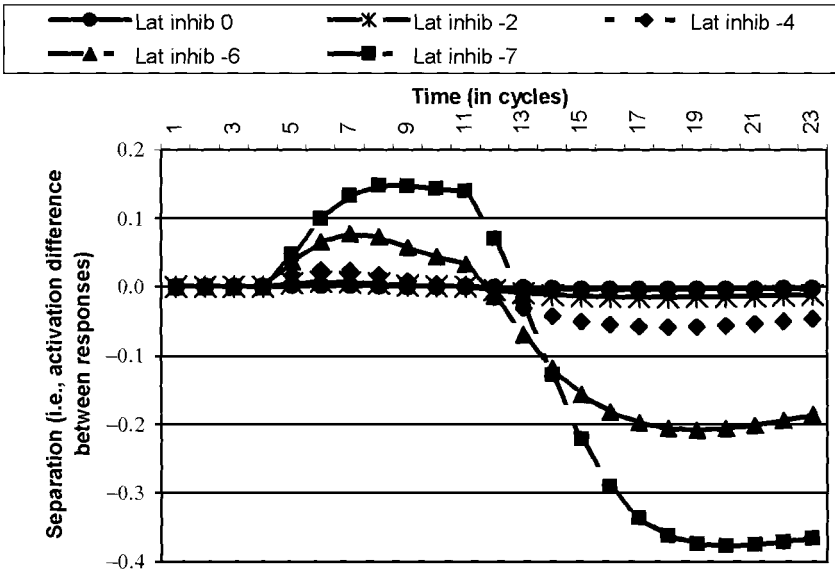
Figure 17. 16.666 ms prime, 100 ms mask, and 100 ms (incompatible) target without opponent process.
