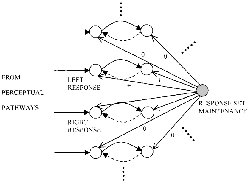
Figure 10. Response-set maintenance (for simplicity of presentation, lateral inhibition between response nodes is not depicted). Links labelled “0” are inactive in this particular experimental condition, thus maintaining the “backgrounding” of irrelevant pathways; links labelled “+” are relaying sustained foregrounding excitation.
