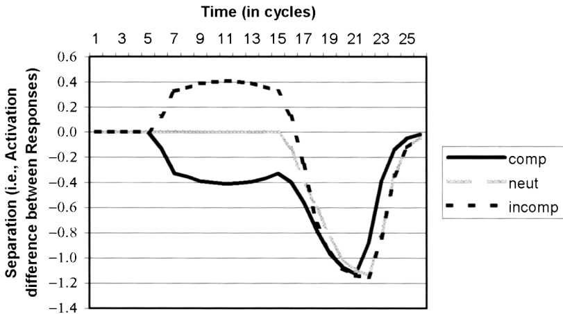
Figure 24. Model separation curves for partial mask, 150 ms ISI experiments.
