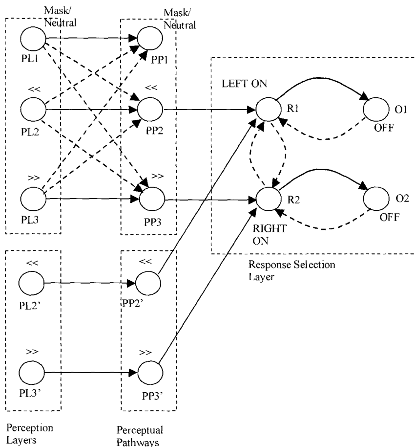
Figure 30. Short prime-target ISI model, with an additional input pathway, which is not subject to feedforward inhibition.
