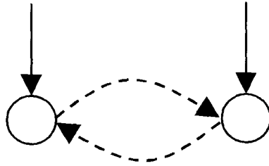
Figure 7. Response system 1.
