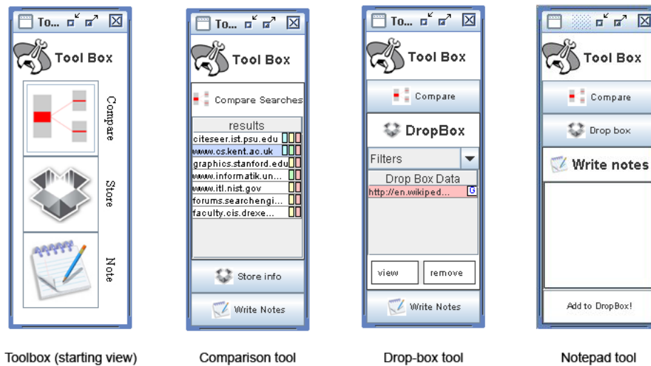
Figure 5.76: The toolbox and its three different tools. This figure shows the starting view of the toolbox (far left), and the views of the three different tools, the comparison tool (centre-left), the drop-box tool (centre-right), and the note-pad tool (far right). When EvoBerry is first activated, the toolbox is displayed in its starting view, but when one of the tools is selected, the view changes to that of the tool. The comparison tool is used to visualize intersections between the multiple searches, the drop-box allows users to add search results for storage, and the note pad allows users to write textual notes (that can be stored in the dropbox).
