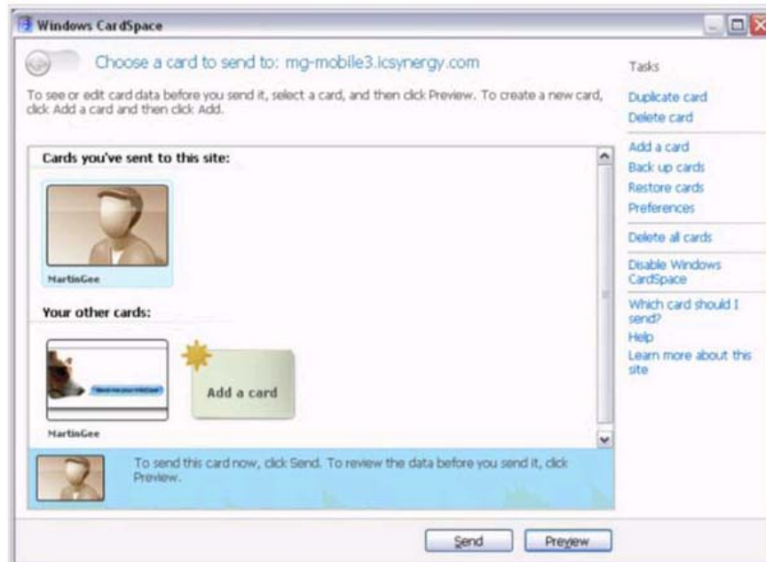
Figure 7. The CardSpace Identity Selector
