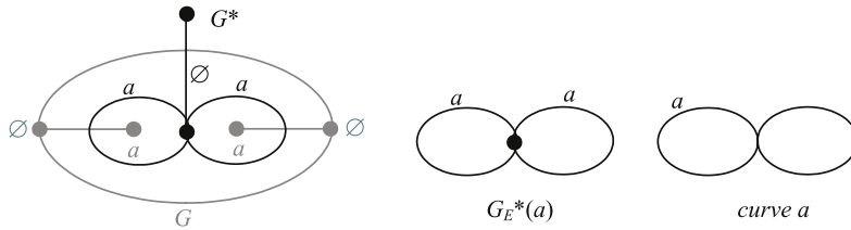
Fig. 15. Converting cycles to curves.
