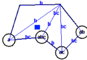
Fig. 28. Ordering labels on dual edges.
