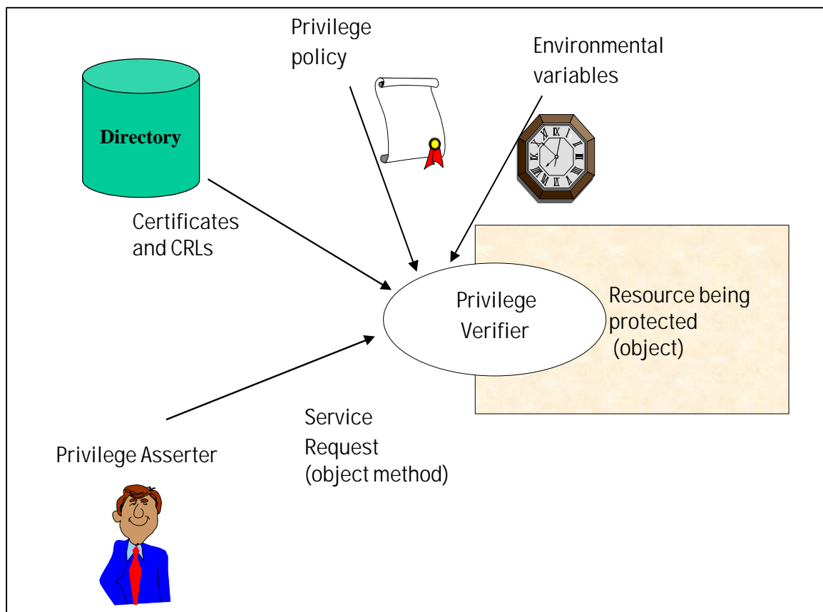
Figure 1. The Privilege Control Model
