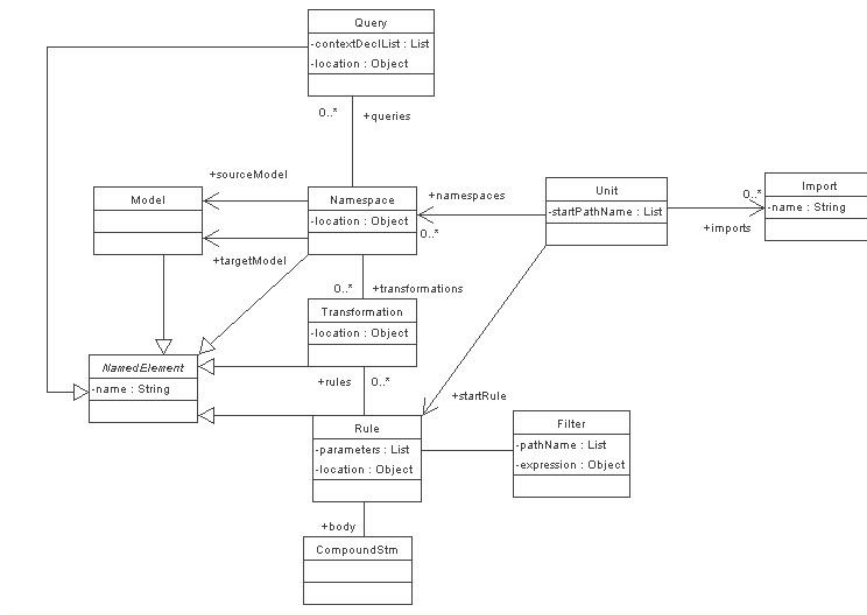
Figure 1 Abstract Syntax
