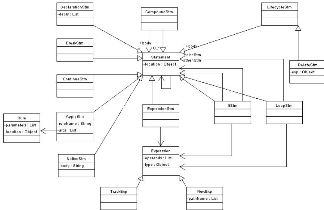
Figure 2 Statements
