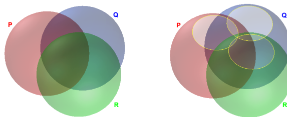
Fig. 4. The necessity of 3-points in 3D.
